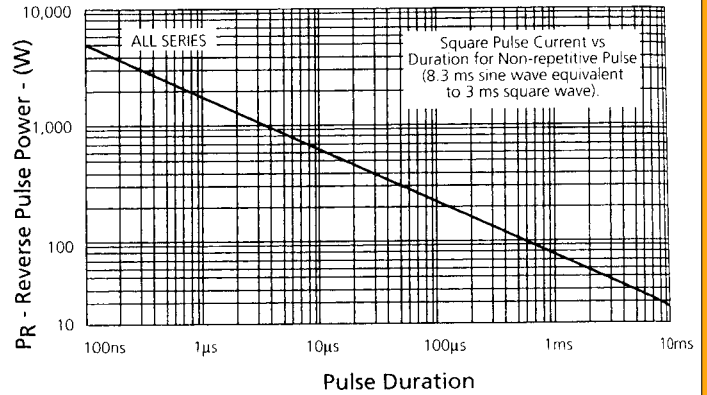
FIGURE 8 Reverse Pulse Power vs. Pulse Duration
